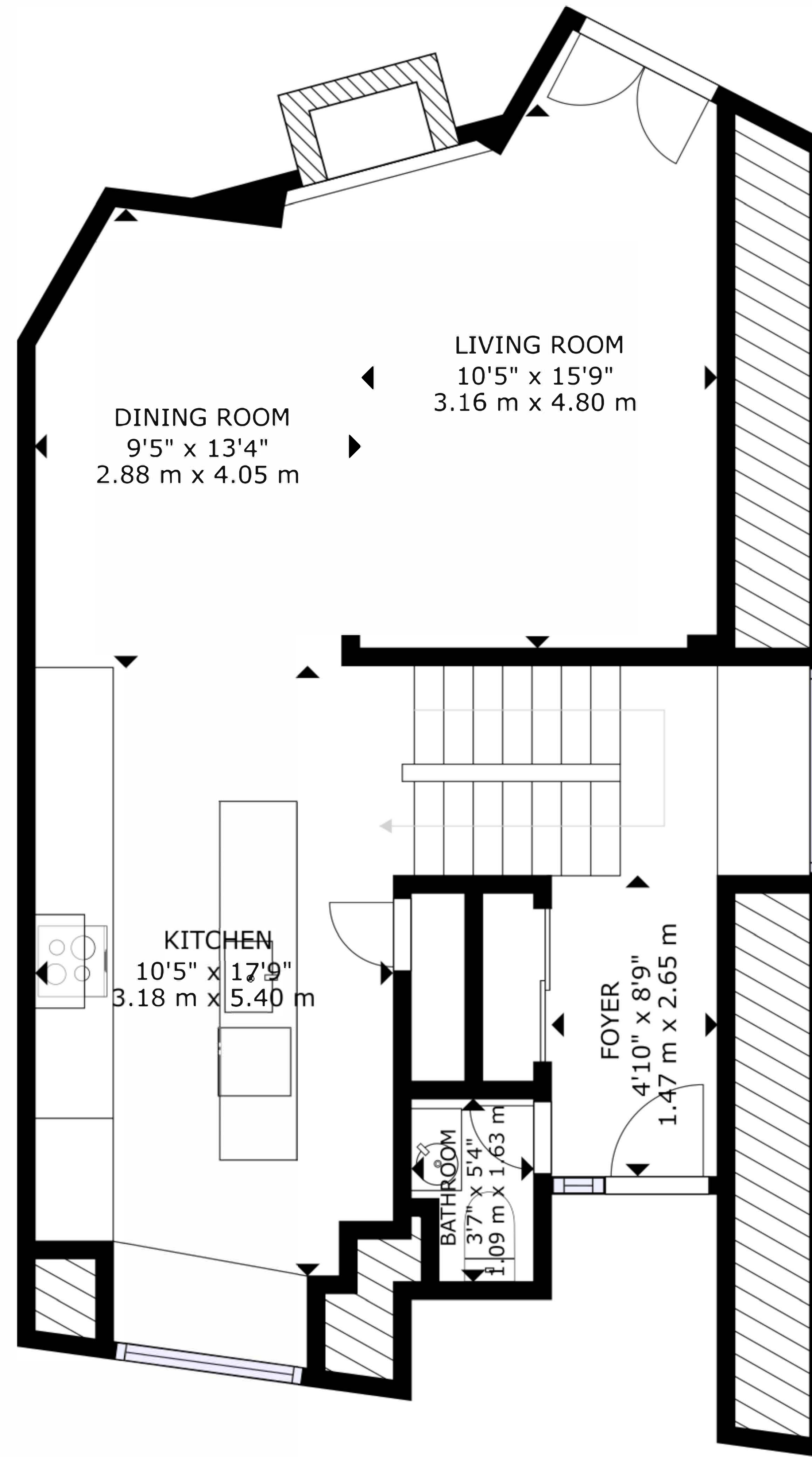
FLOOR 2
